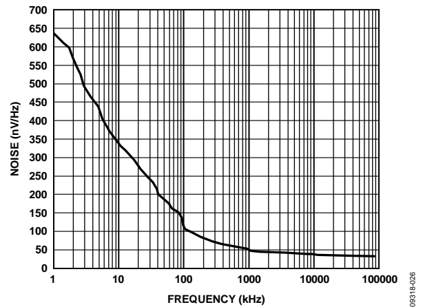
Figure 29. ADV3229 Output Noise, 100 \Omega Load
