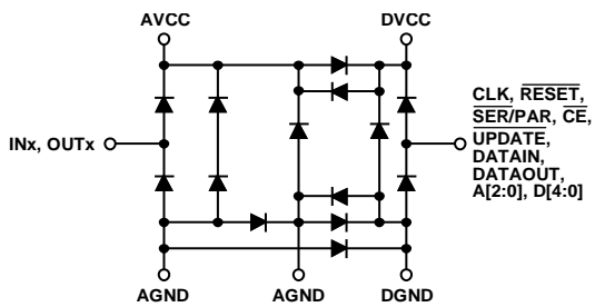
Figure 60. ESD Map
