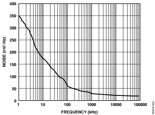
Figure 26. ADV3228 Output Noise, 100 \Omega Load
